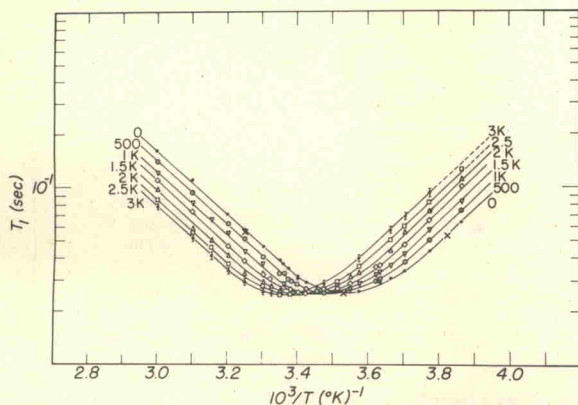
FIG. 1. T_1 as a function of temperature with pressure a parameter at 30 MHz for glycerol. The \times represents atmospheric data taken from Connor, Ref. 27.
